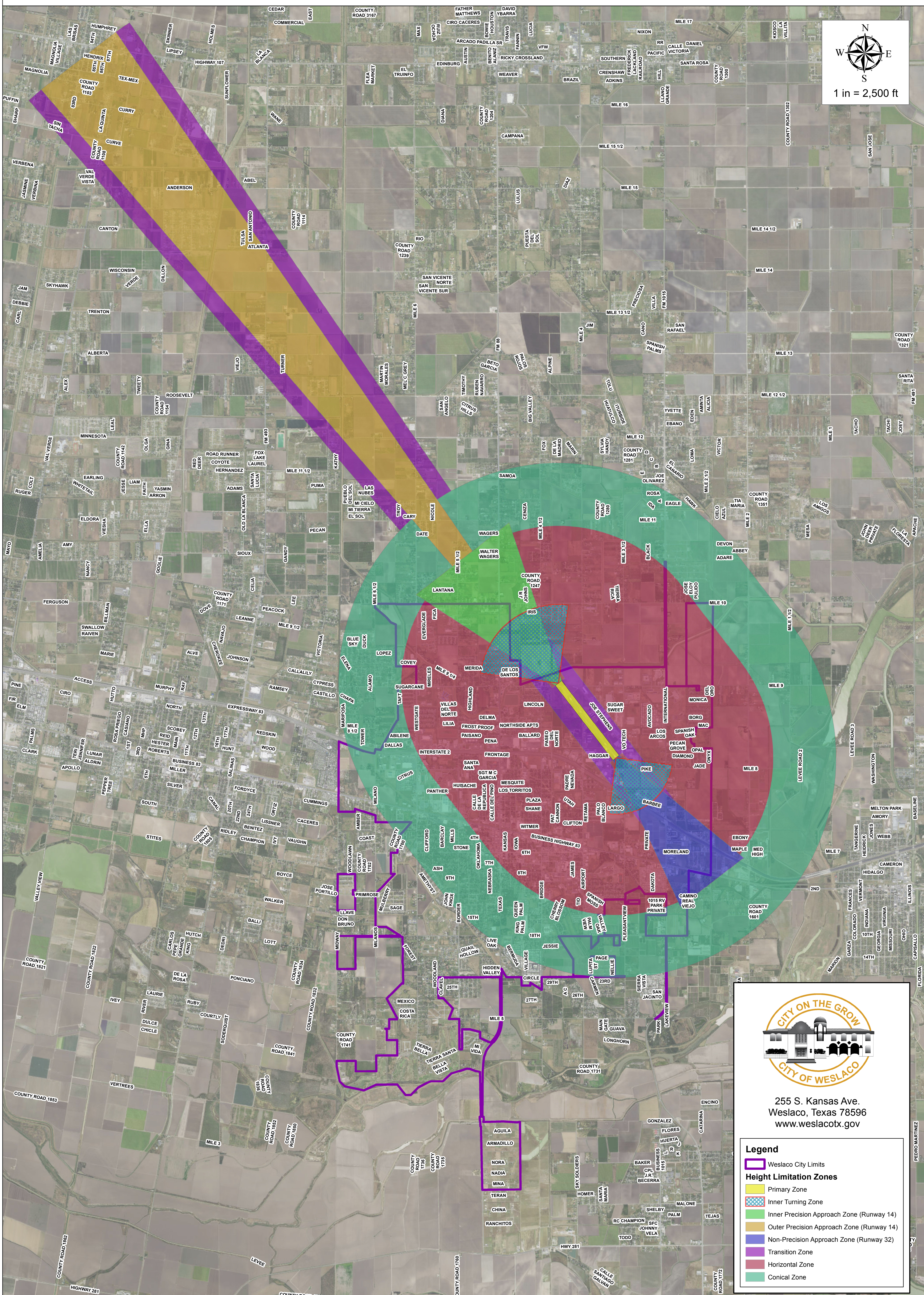
MID VALLEY VALLEY AIRPORT HEIGHT LIMITATIONS ZONES FIGURE 1
